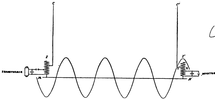
FIG. 3.—THEORY OF WIRELESS TELEGRAPHY.
